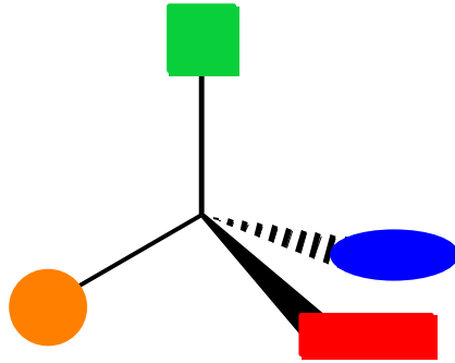
Molecule A
