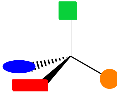
Molecule B
